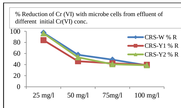
Fig. 7: Optimization of initial Cr(VI) concentration in the effluent for its effective reduction using microbe cells (Initial Conc. Vs % Reduction of Cr(VI))
