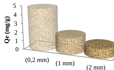
Figure 5: Particle size effect on nitrate adsorption
