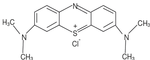
Fig. 1: Chemical structure of MB dye
