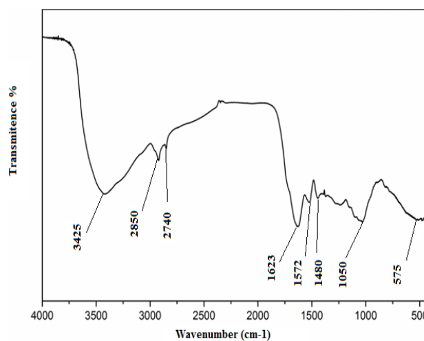
Fig. 2: FTIR spectra of Grape Marc in the range from 4000 to 500 \text{cm}^{-1}
