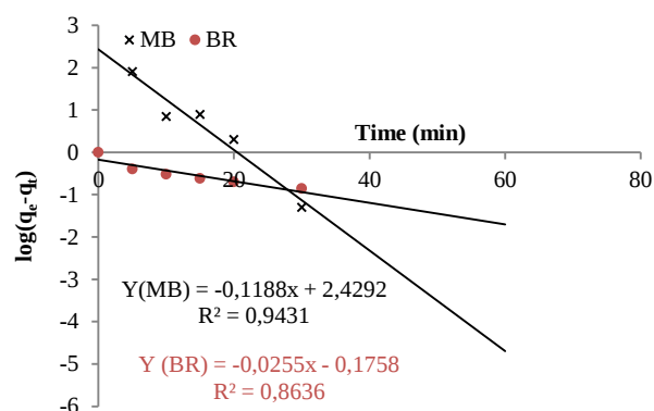
Fig. 9: Pseudo-first order plot for the adsorption of MB and BR on GM waste
