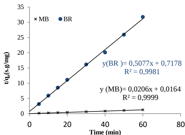
Fig. 10: Pseudo-second order plot for the adsorption of MB and BR on GM waste
