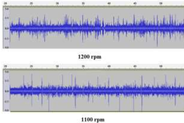
Figure 8: Analysis of recorded sounds from the primary extractor at 1100 and 1200 rpm
