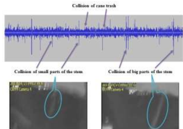
Figure 7: Results obtained from the analysis and adaptation of recorded sounds from inside the sugarcane harvester primary extractor hood chamber and related camera videos
