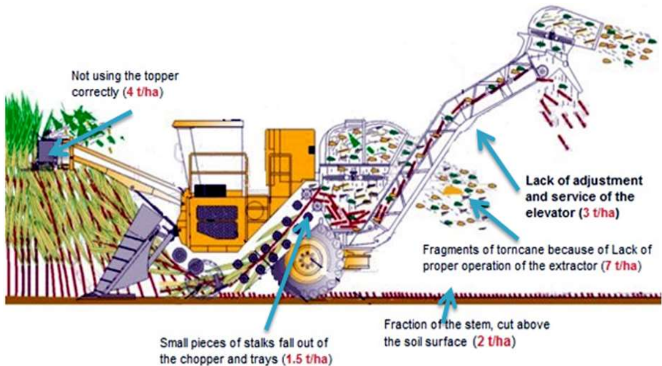
Figure.1: Most non-recyclable losses and sources of its creation in a modern sugarcane harvester in Iran
