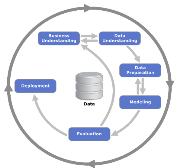
Figure 3: CRISP-DM Cycle
