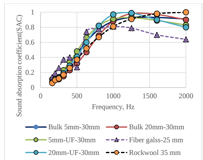
Figure 14: Comparison of sound absorption of NAF absorber samples with rockwool and fibreglass.
