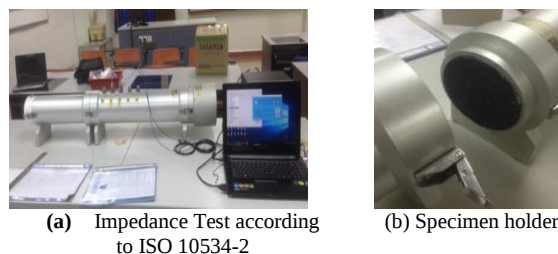
Figure 6: Sound absorption test
