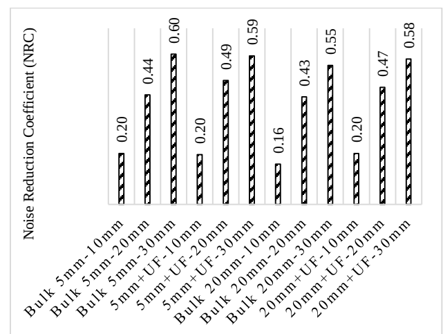
Figure 13: NRC of absorber samples with fiber size of 5 and 20mm for thickness of 10mm, 20mm, and 30mm with and without binder.
