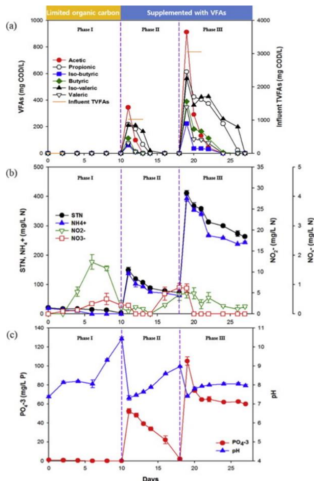
Figure 3: Changes of chemical components in consortium of microalgae and bacterial with stepwise increment of biologically produced volatile fatty acids circulating within the photobioreactor: (a) VFAs, (b) STN, \text{NH}_4^+ , \text{NO}_2^- , and \text{NO}_3^- , (c) pH and \text{PO}_4^{3-} . Ad Adopted from [68]
