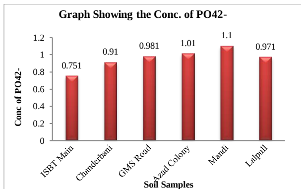
Figure 2: \text{PO}_4^{2-} ion in Various Soil Samples at Region 1
