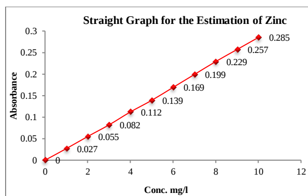
Figure 13: Standard Graph for the estimation of Zinc
