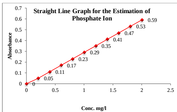
Figure 1: Standard Graph for the estimation of \text{PO}_4^{2-}
