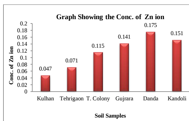
Figure 15: Zn 2+ ion in Various Soil Samples at Region 2
