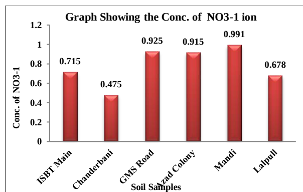
Figure 5: \text{NO}_3^{1-} ion in Various Soil Samples at Region 1
