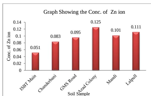
Figure 14: Zn 2+ ion in Various Soil Samples at Region 1
