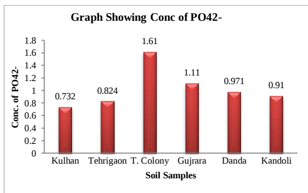
Figure 3: \text{PO}_4^{2-} ion in Various Soil Samples at Region 2
