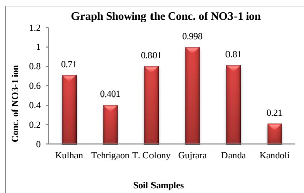
Figure 6: \text{NO}_3^{1-} ion in Various Soil Samples at Region 2
