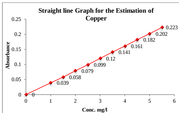
Figure 16: Standard Graph for the estimation of Copper
